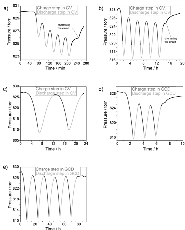
Figure 2. a–e) Pressure changes observed during cyclic voltammetric and galvanostatic charge (dark gray) and discharge (light gray) at 1 (a), 0.2 (b), and 0.05 mV s −1 (c), as well as at 10 (d) and 2 mA (e).
